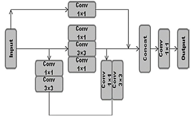
Fig. 3. The architecture of ResNet[25]
