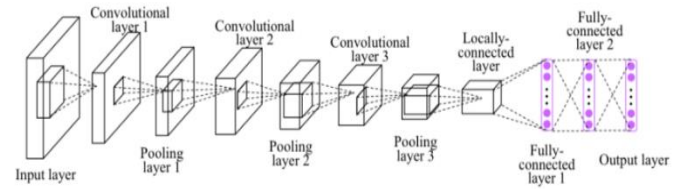
Fig. 4. Architecture of CNN[34].
